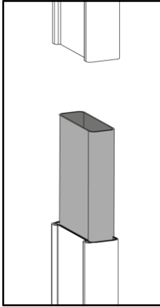
Holminnenverbinder Aluminium 60 x 20
