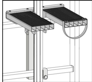
Ruhepodest SP 305 x 140
