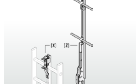
Einstiegshilfe H-50.2 Plug-in device H-50.2
