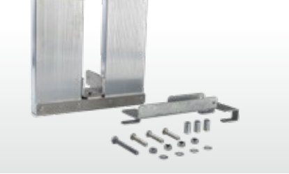
Ruhepodest SP 305x140 T-Anbindung Resting platform SP 305x140 T-connection
